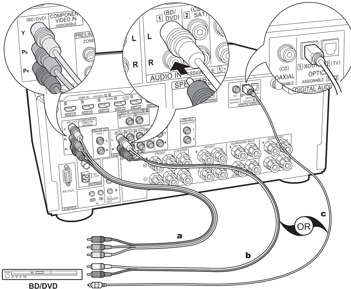
a Component Video Cable, b Analog Audio Cable, c Digital Optical Cable
